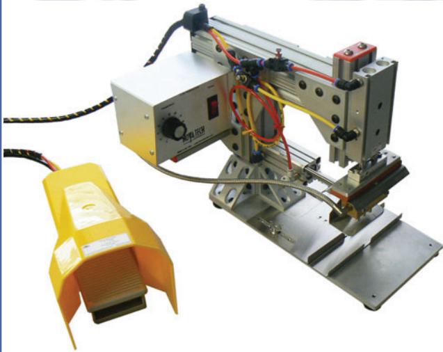
Model shown: RX-95-PM2-RK Multi Hole Punch with basic controller and optional slug-catch tray (shown with safety guard below)
