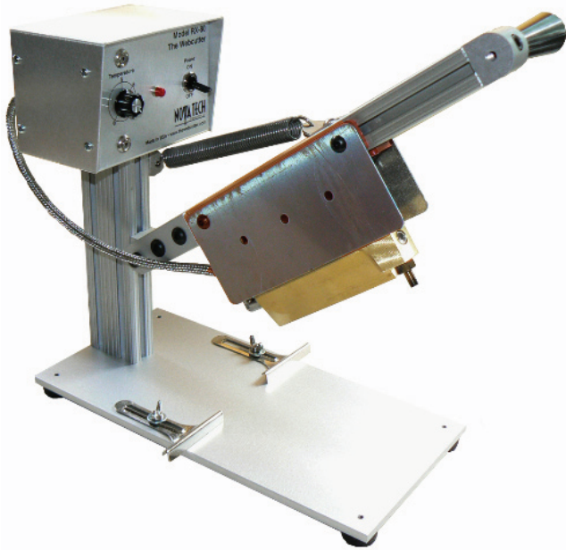
Model shown: RX-80-BHL-RK 4" (110mm) Brass Hot knife with interchangeable Punch Collet (see custom configurations on back)
