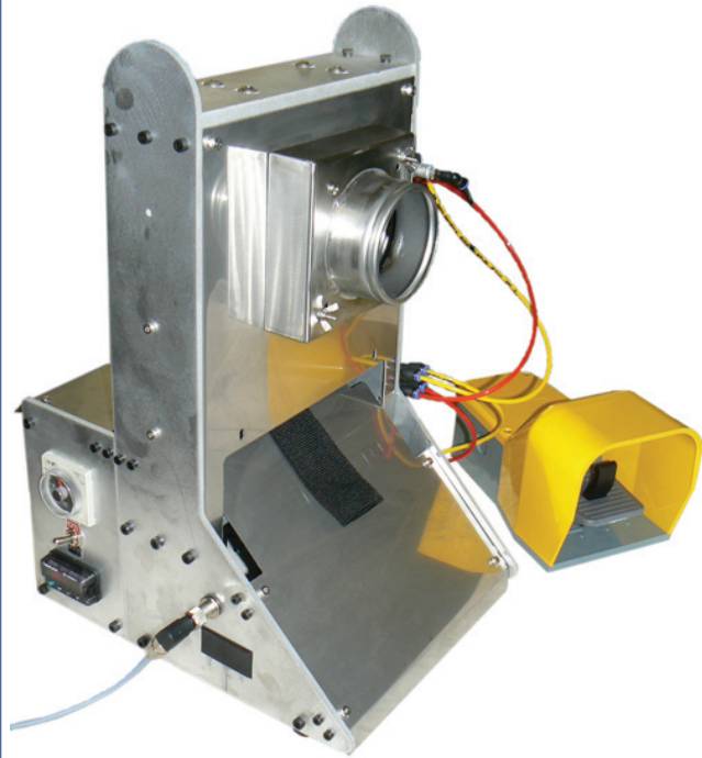
Model shown: RX-92-SCT-TK 5" (130mm) Pneumatic Hot Knife with PID Temperature Control and Adjustable Dwell Timer, 120V (see custom configurations on back)
