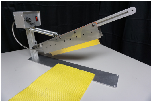
Model below: RX-84-BAO-RK 13" (330mm) Heavy-duty Brass Hot Knife
